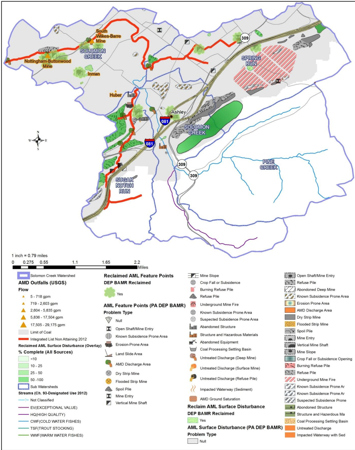
Figure 2-14 Abandoned Mine Lands and Mine Drainage Impacts to the Solomon Creek Watershed
