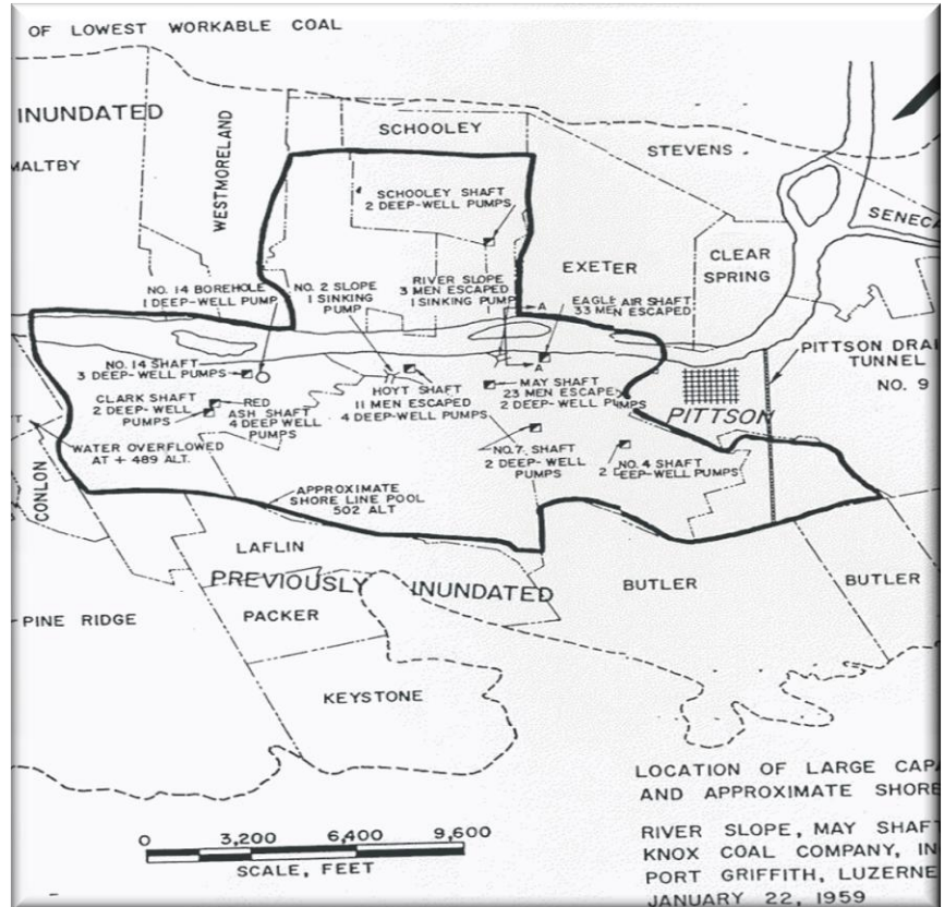
Figure 2-32 Knox Mine Disaster Pump Stations and places where men escaped, 1959
