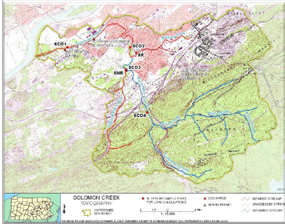
Figure 2-27 In stream Sampling Points for Load Calculations and Discharge Points, along with the categories of the stream impairments within the Solomon Creek Watershed (Solomon Creek TMDL Report, 2007)
