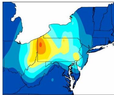
Figure 2-22 (Above) Annual pH from 1983 - 1994
