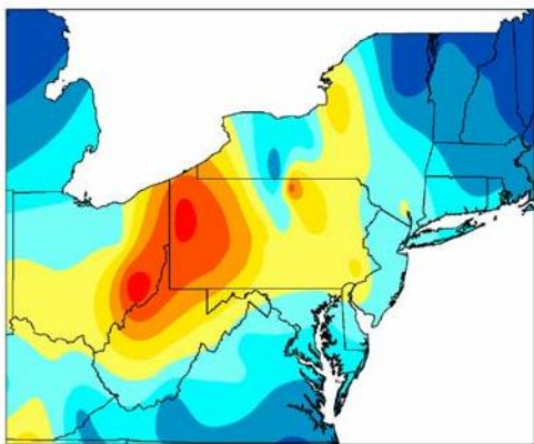
Figure 2-23 (Above) Annual Sulfate Deposition (kg/ha) from 1983 - 1994
