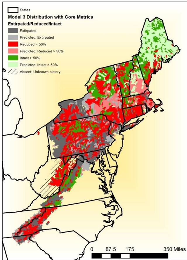
Figure 3-2 Model 3 Distribution of Trout Populations with Core Metrics (EBTJV, 2006)
