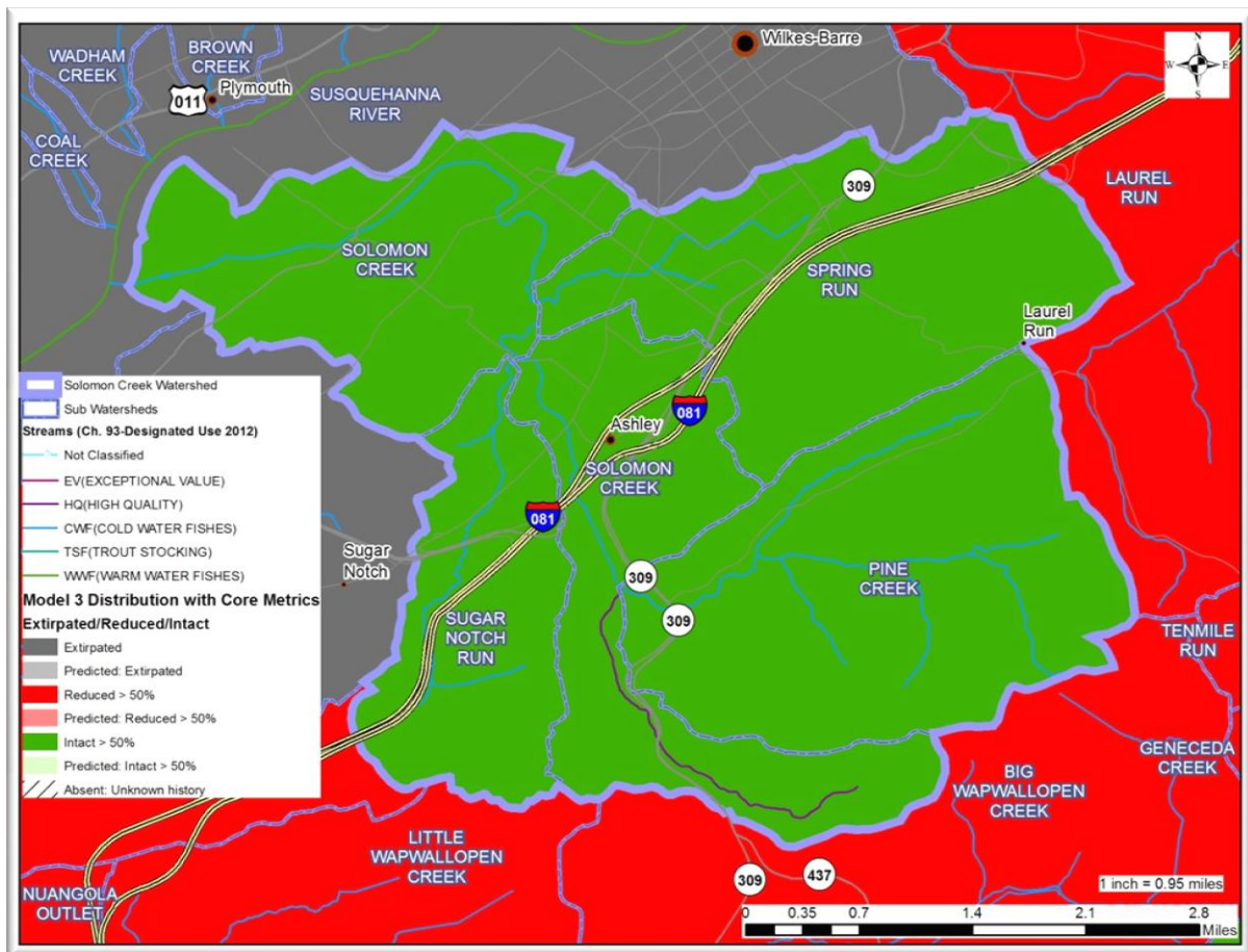
Figure 3-3 Solomon Creek Model 3 Distribution with Core Metrics and Surrounding Streams (EBTJV, 2006)
